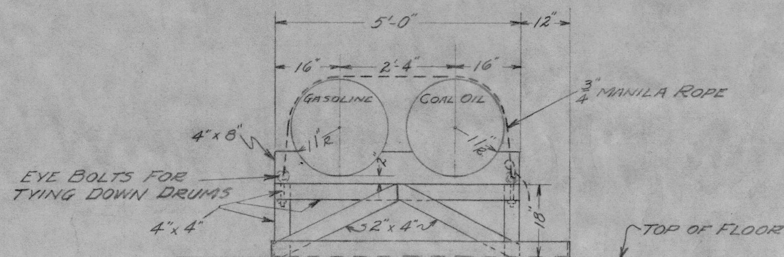
VIEW B-B
