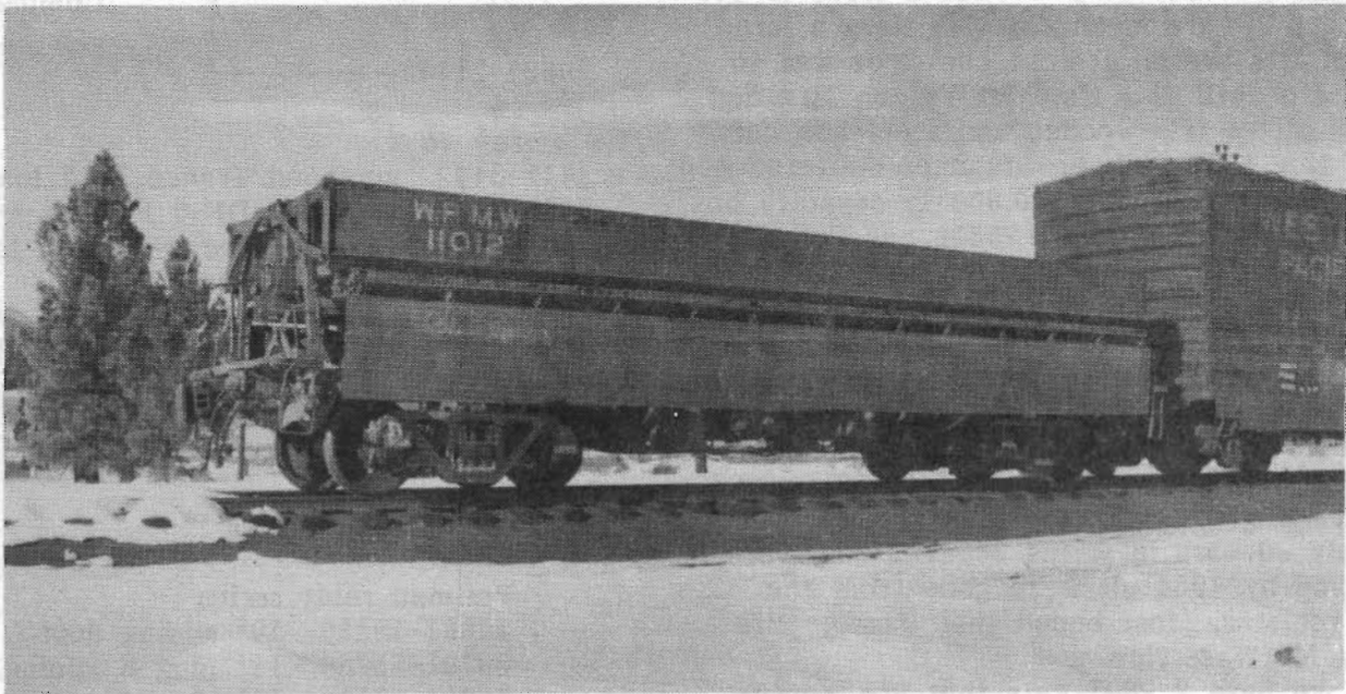
DUMP CAR CAR NOS. 11001-11040 BUILT BY WESTERN WHEELED SCRAPER CO. , ORIG. NO. OF CARS. 40. AURORA, ILL. JUNE, 1927.
